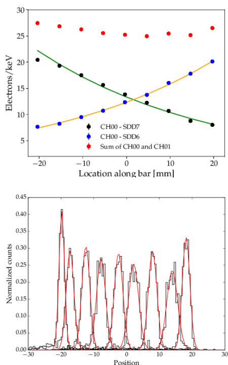
Fig. 9. Upper panel: Light attenuation along the bar. The signal from both detectors is shown, together with a best-fit exponential attenuation line. Lower panel: Reconstructed position for various measurements along the bar.
